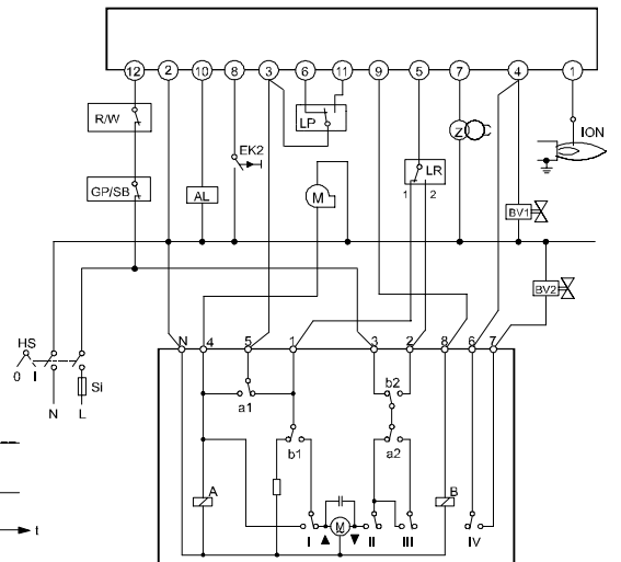
SQN7x.424xx / 2-stage control 2-wire control
