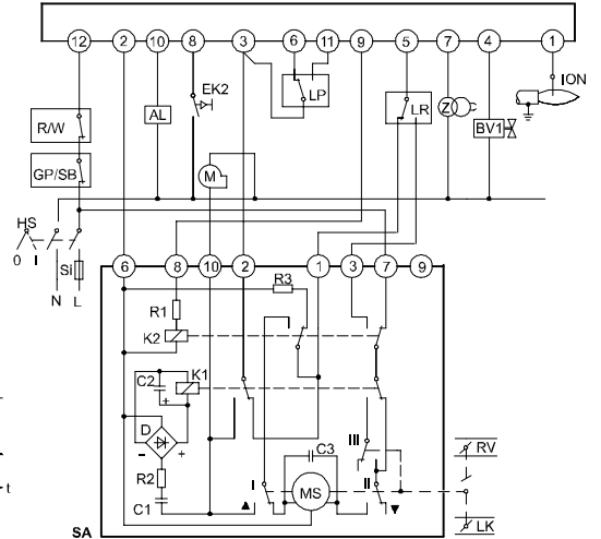
SQN90.220x / 2-stage modulating control
