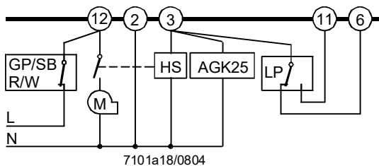
Only for burner with fan control via auxiliary contactor (HS) with air pressure switch (LP)
