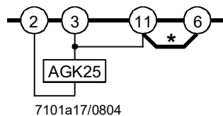
Burner without fan and without air pressure switch (LP)
